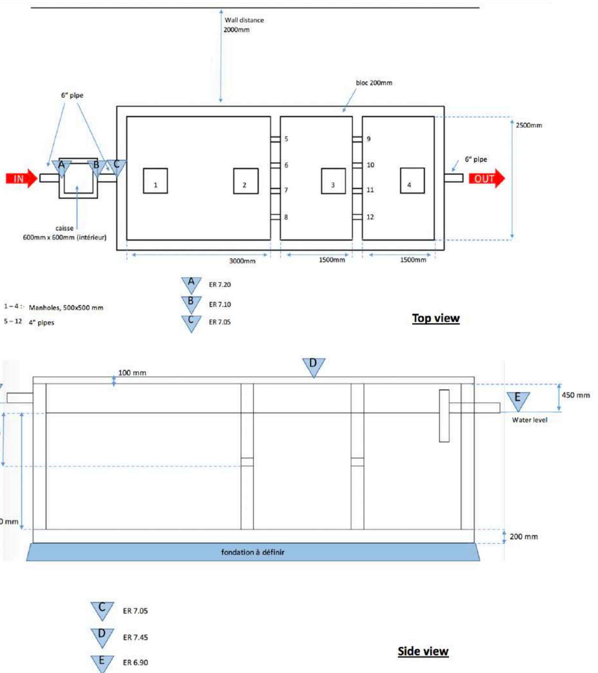
Figure 29: detailed drawing of the septic tank, top and side view
